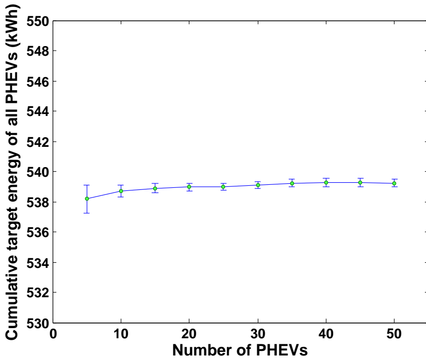
Figure 14. Comparison of the cumulative target energy allocated to all PHEVs in different cases.
