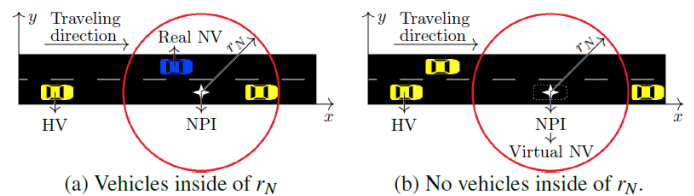
Fig. 1. NV location: a) the closest vehicle to the NPI inside a radius r_N is chosen as the NV (the blue one), and b) a virtual vehicle is chosen.
